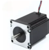
NEMA23 Stepper Motor 57x82mm 4.2A 2.2N.m 57HS82-4204
