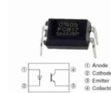
PC817 pin 4 Optocoupleur phototransistor
